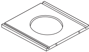
B-298x273x12mm(1pc)
