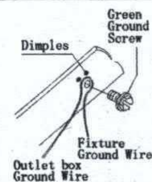
Grounding Detail
