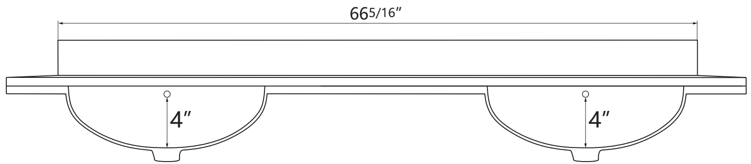
Front View
