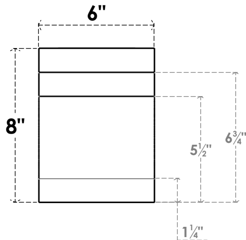
FRONT PROFILE
