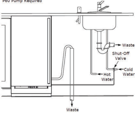
Stand Pipe P60 Pump Required
