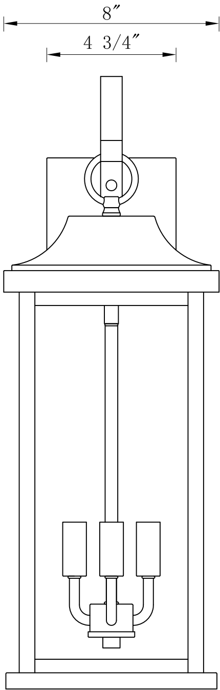
FRONT VIEW
