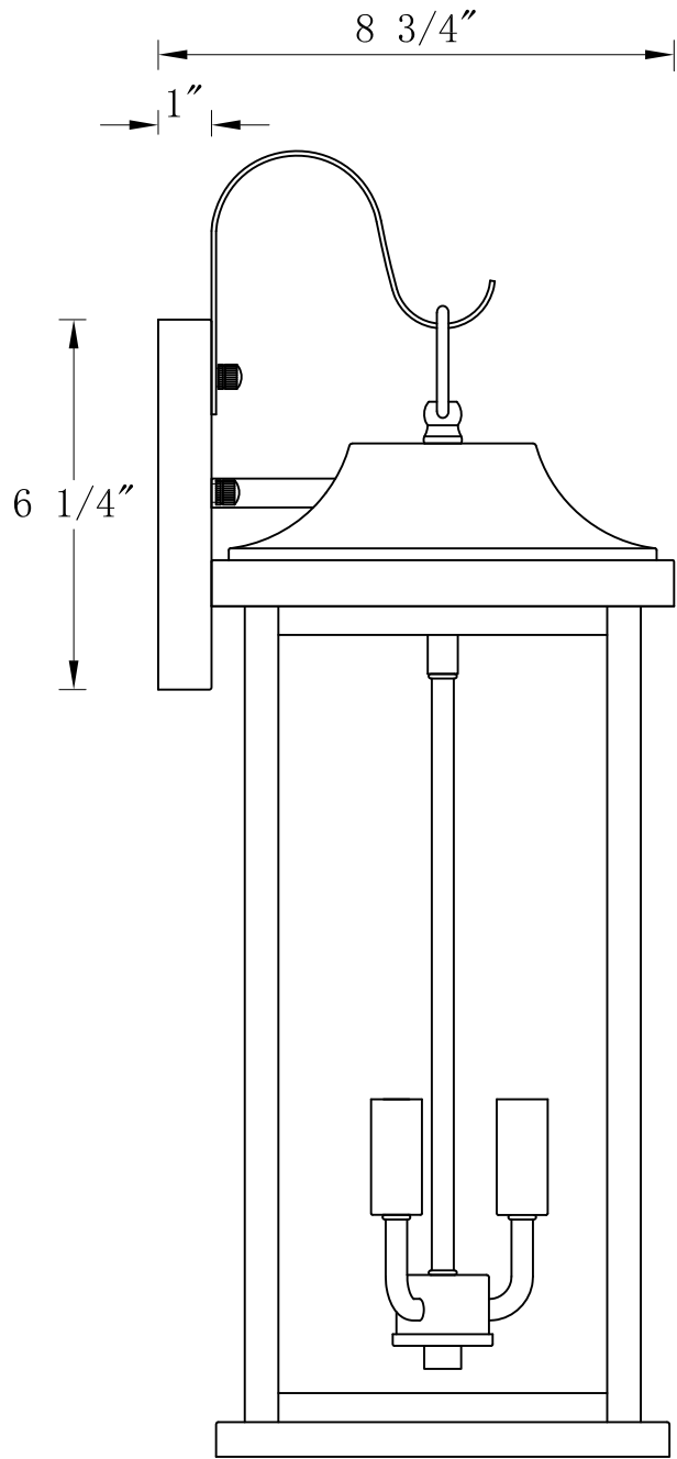
SIDE VIEW
