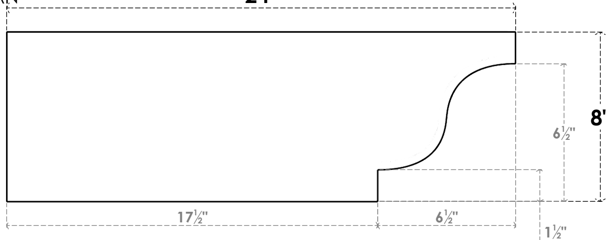
SIDE PROFILE
