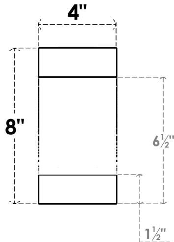
FRONT PROFILE
