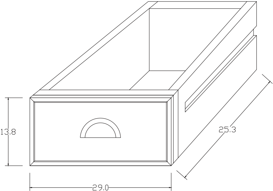
DRAWER DESIGN
