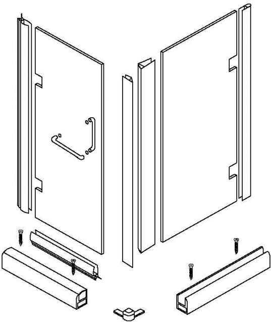
RIGHT DOOR INSTALLATION
