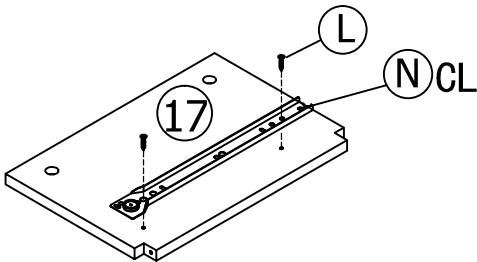
Right side
