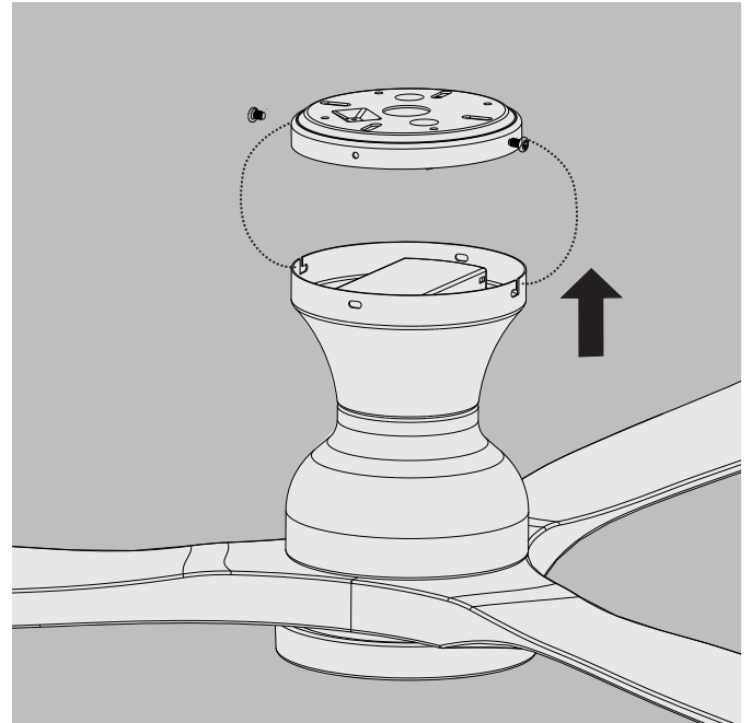
❷ Insert the ceiling fan into the gap position
