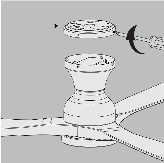
❶ Install the screws on both sides of the hanging disc (leave 3-5mm)
