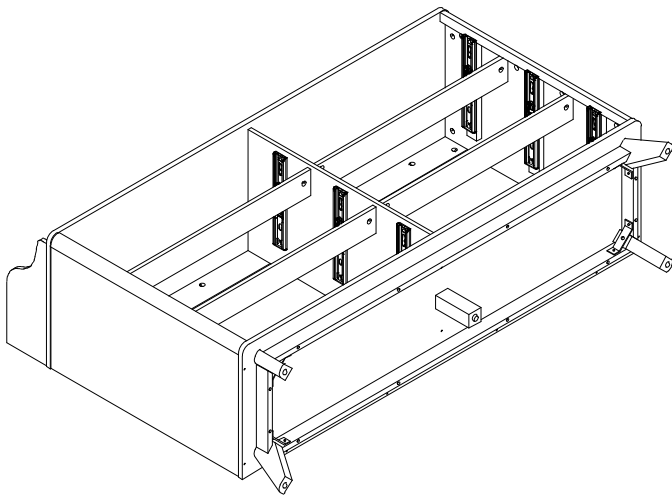
Completed Assembly
