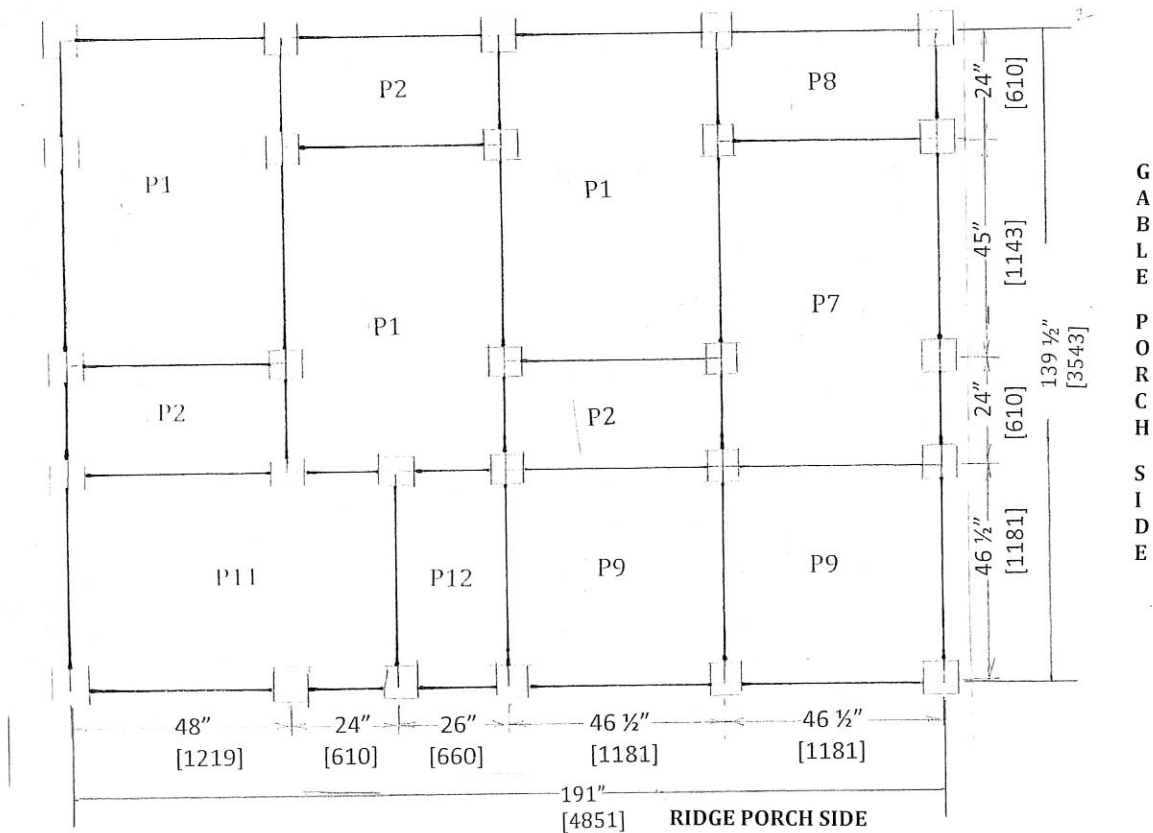
RIGHT WRAP AROUND JOIST BOX CONFIGURATION
