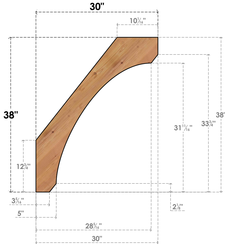
SIDE
