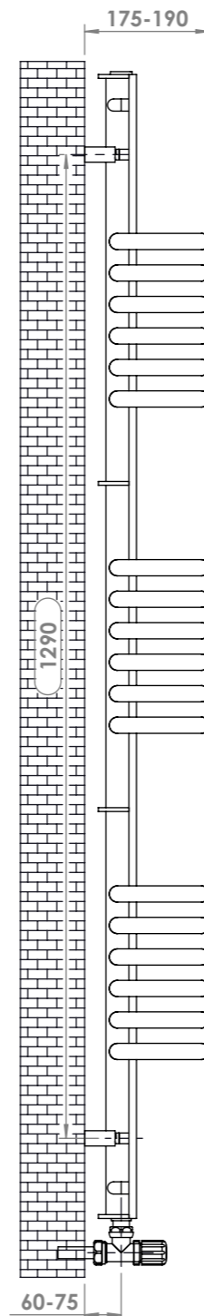
Side View
