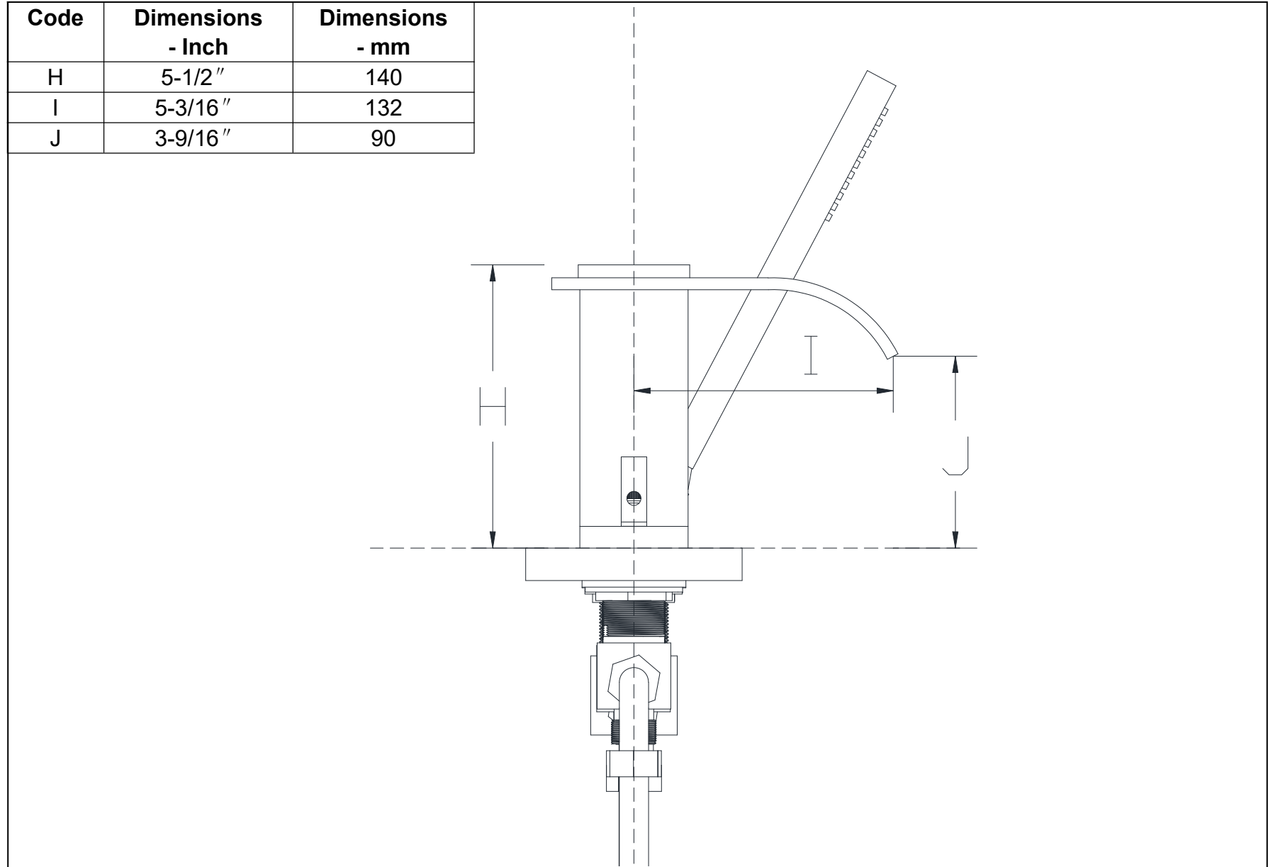
Side View
