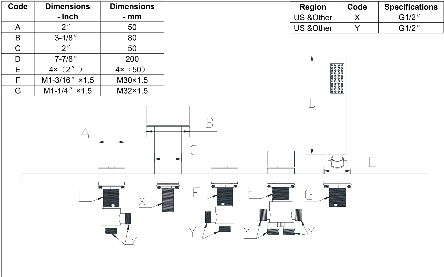
Front View
