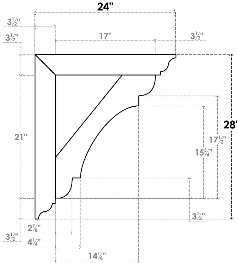
SIDE PROFILE
