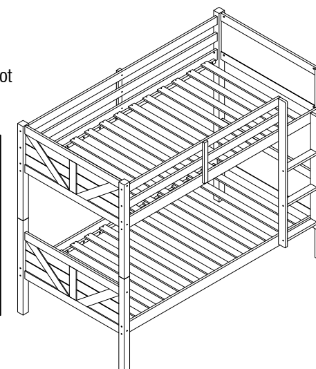
(M) Sets of Slats x 2
