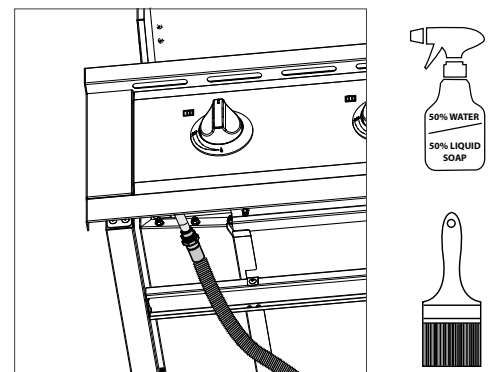
Leak Testing Diagram
