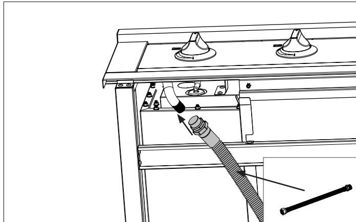
Metal Corrugated Extension Hose + PVC Natural Gas Hose
