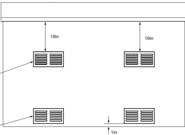
Back View
