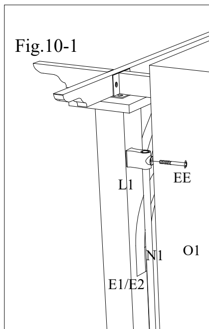
Fig.10-1: First, insert the canopy rod 1/ canopy rod 1 (M1/M2) into the rail beam (N1), then insert the rail beam (N1) into the rail connector (L1), finally lock rail beam (N1), connector (L1) and post (E1/E2) by using bolt (EE).
