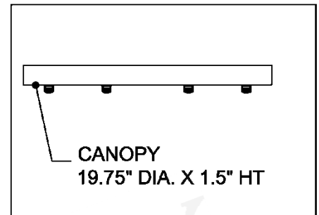
CANOPY DETAIL
