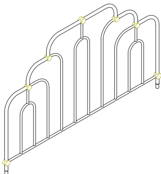
① Headboard 1595x25.4x972mm (1)
