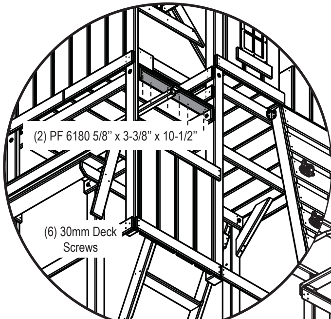
Under Deck View
