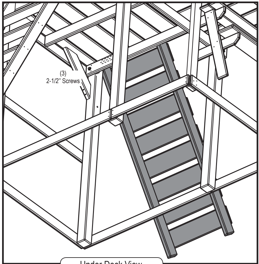
Under Deck View
