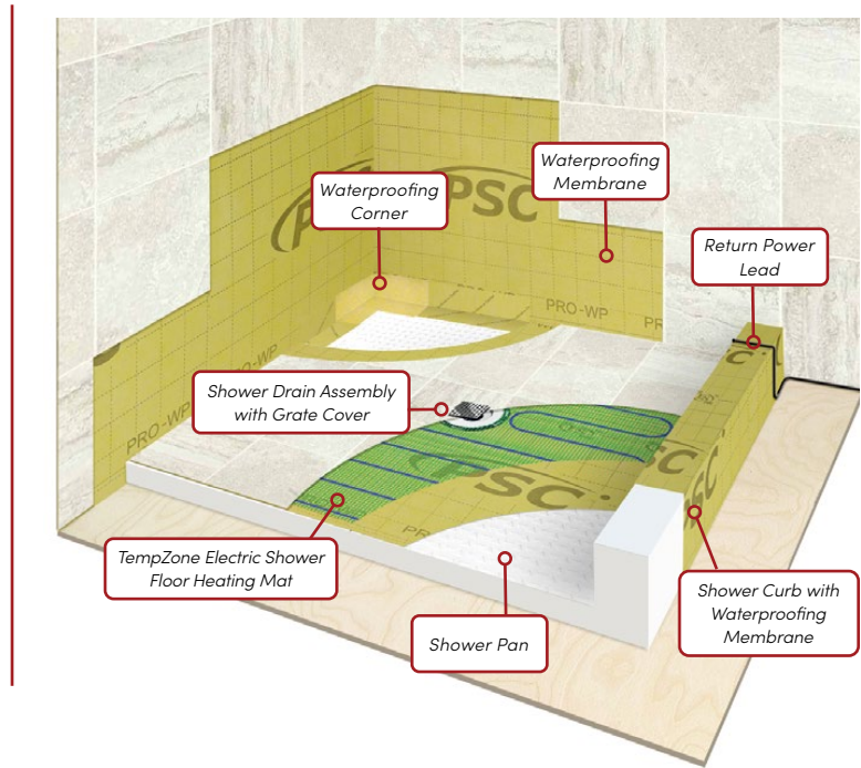
TempZone Electric Shower Floor Heating Kit includes a TempZone Electric Shower Floor Heating Mat, Circuit Check, and Programmable Thermostat
