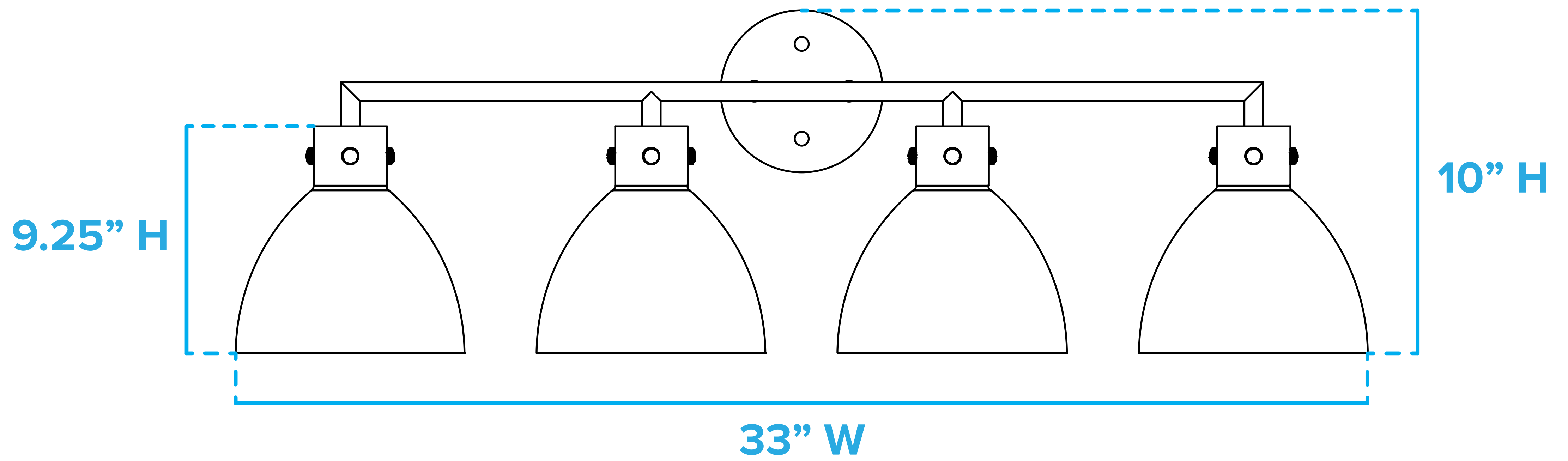
Front View
