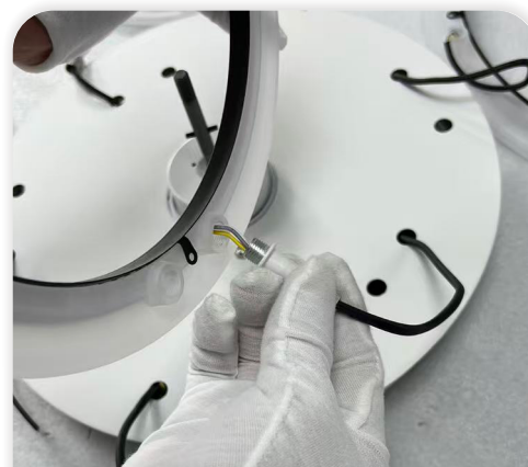
3 Align with the threaded hole and tighten
