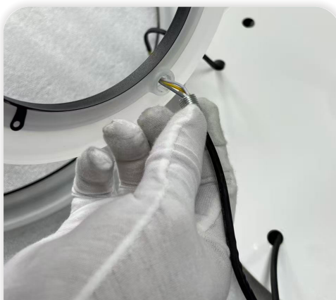
2 Pass the nipple screw through the lamp holder wire
