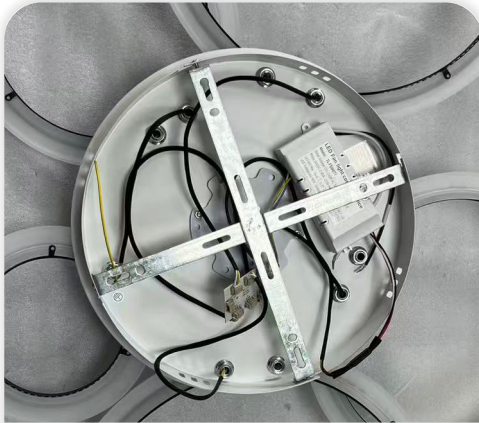
16 Check and tighten the other four screws.
