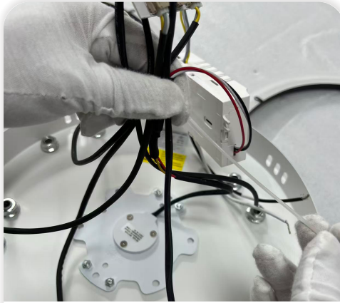
14 Use cable ties to bundle the wires.
