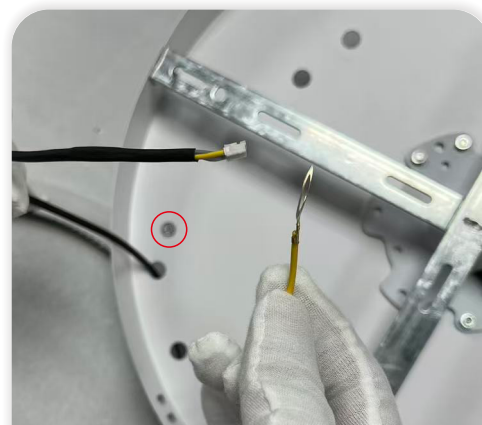
9 Locate the hole marked for the ground wire.
