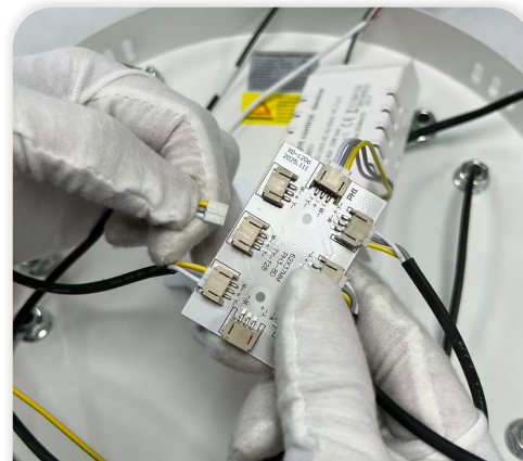
12 Insert the wires of the other lamp holders in sequence.
