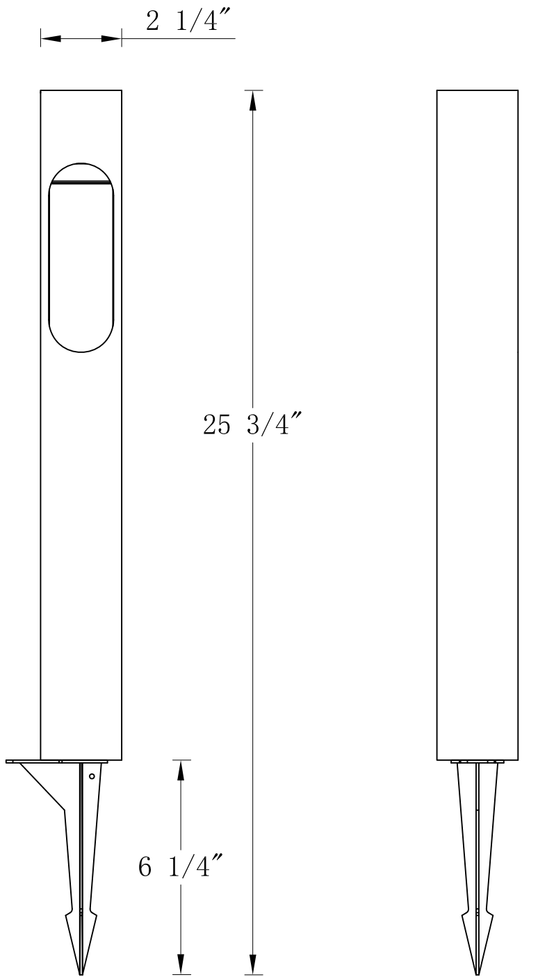
FRONT VIEW
