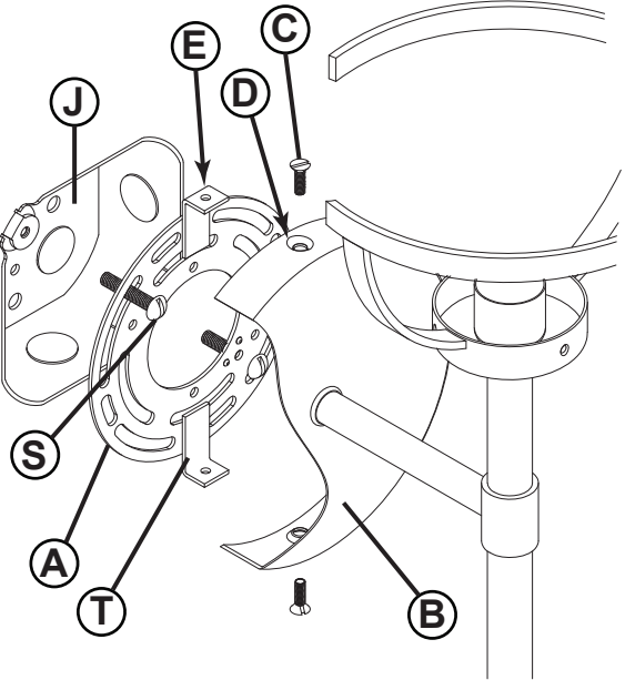
DRAWING 1 - GLASS INSTALLATION
