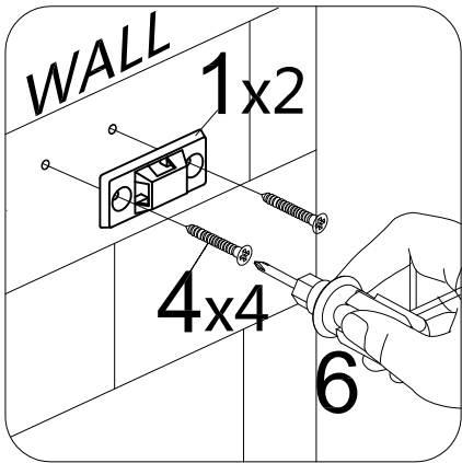
3.Secure the Anti-tip device ① to the wall with screws ④ .
