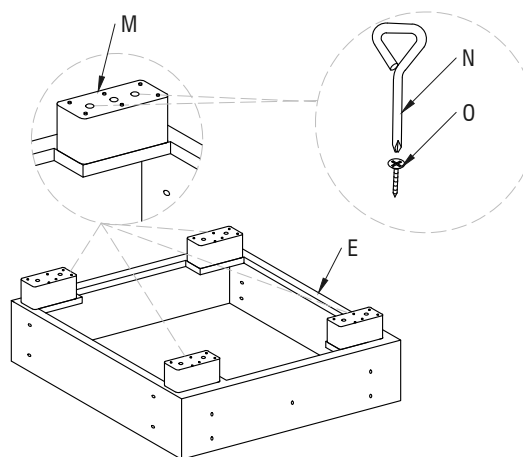
Plastic leg M through N/O fixed on base E
