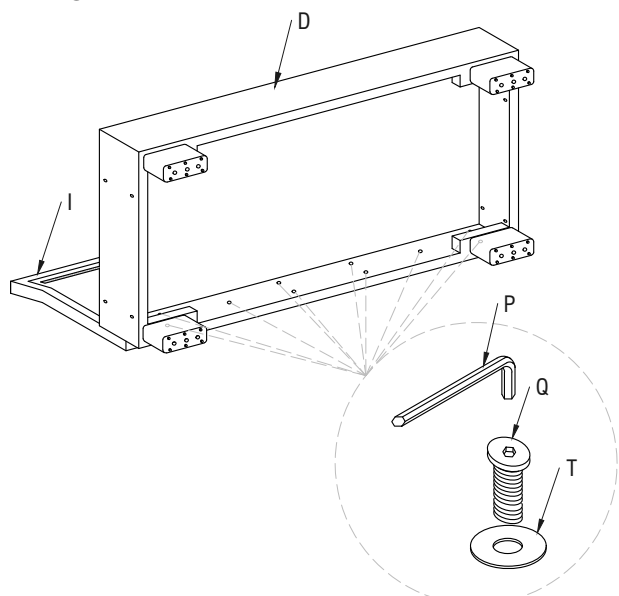
Through P/R/T fixed on base D and back I
