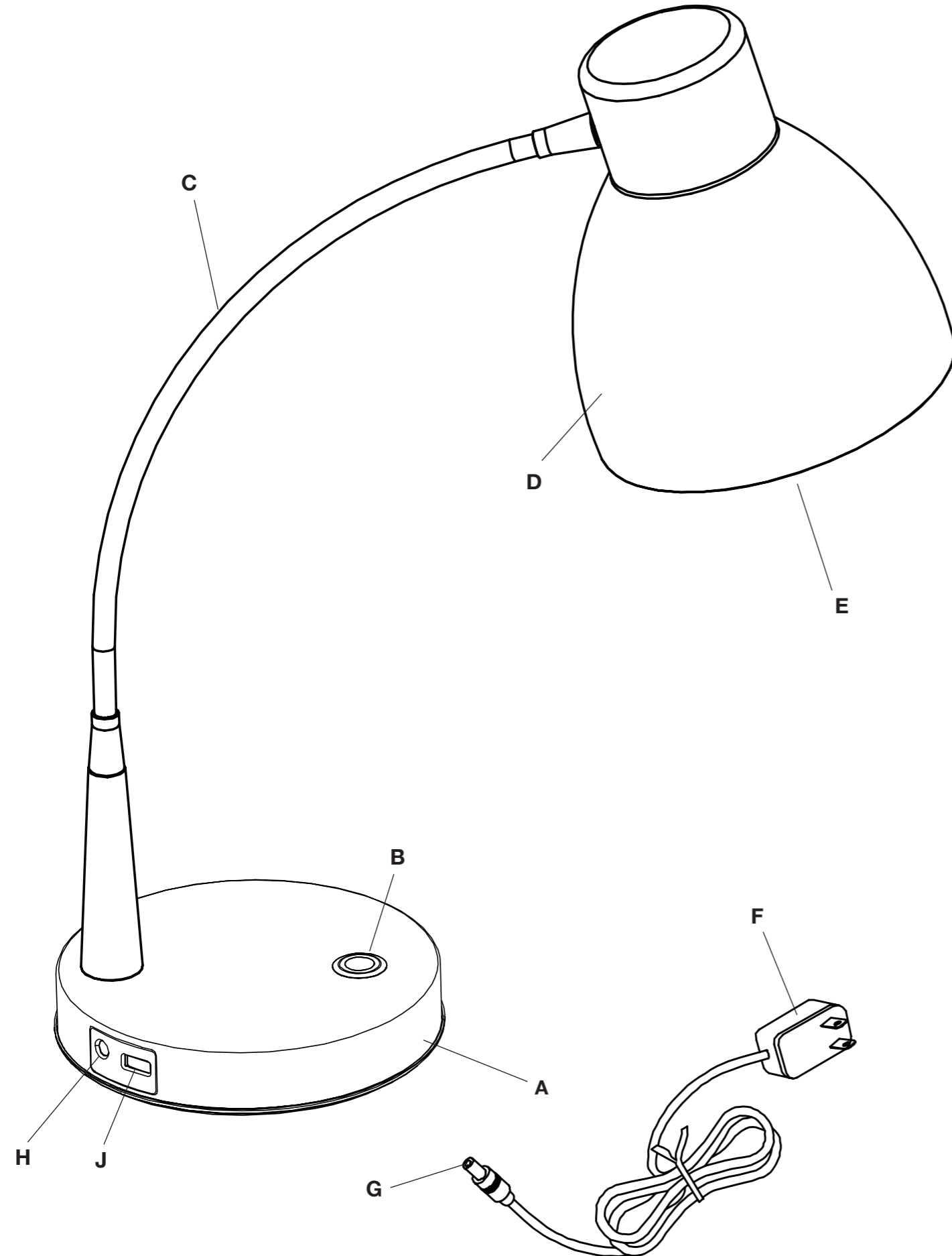
Adjust LED Desk Lamp with USB
