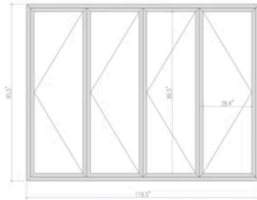
Front View Dimension
