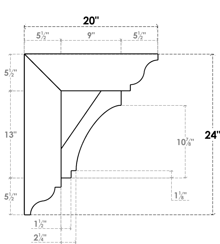
SIDE PROFILE
