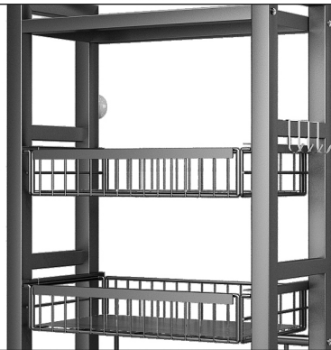
5. Install the hook
