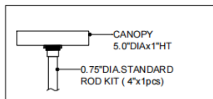
CANOPY DETAIL
