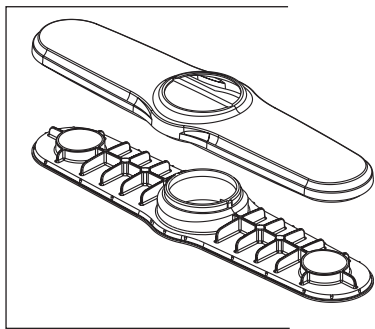
RP101142▲ (Escutcheon optional, not included) Escutcheon & Base Plate (3 Hole) Chapetón y Placa de Base (3 agujeros) Boîtier et Plaque de Finition (3 trous)
