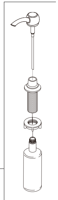
RP70710▲ (Dispenser optional, not included) Dispenser Assembly (complete) Ensamble del Surtidor (completo) Distributeur (complet)
