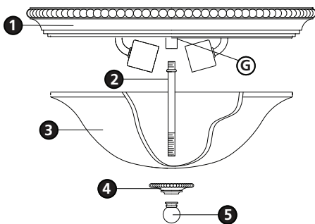
Drawing 3 - Glass Installation
