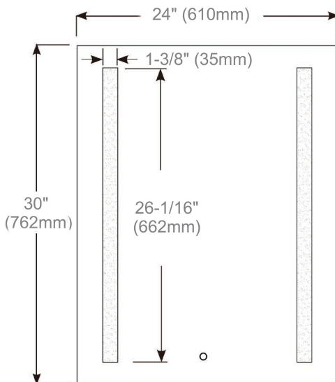
Cabinet Dimensions
