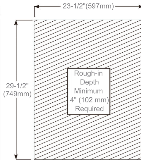
Rough-in Dimensions
