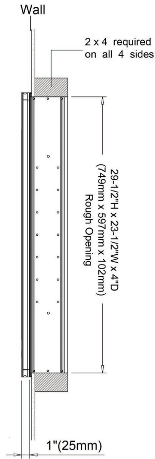
Recessed Mount
