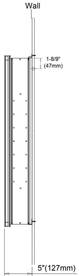
Surface Mount
