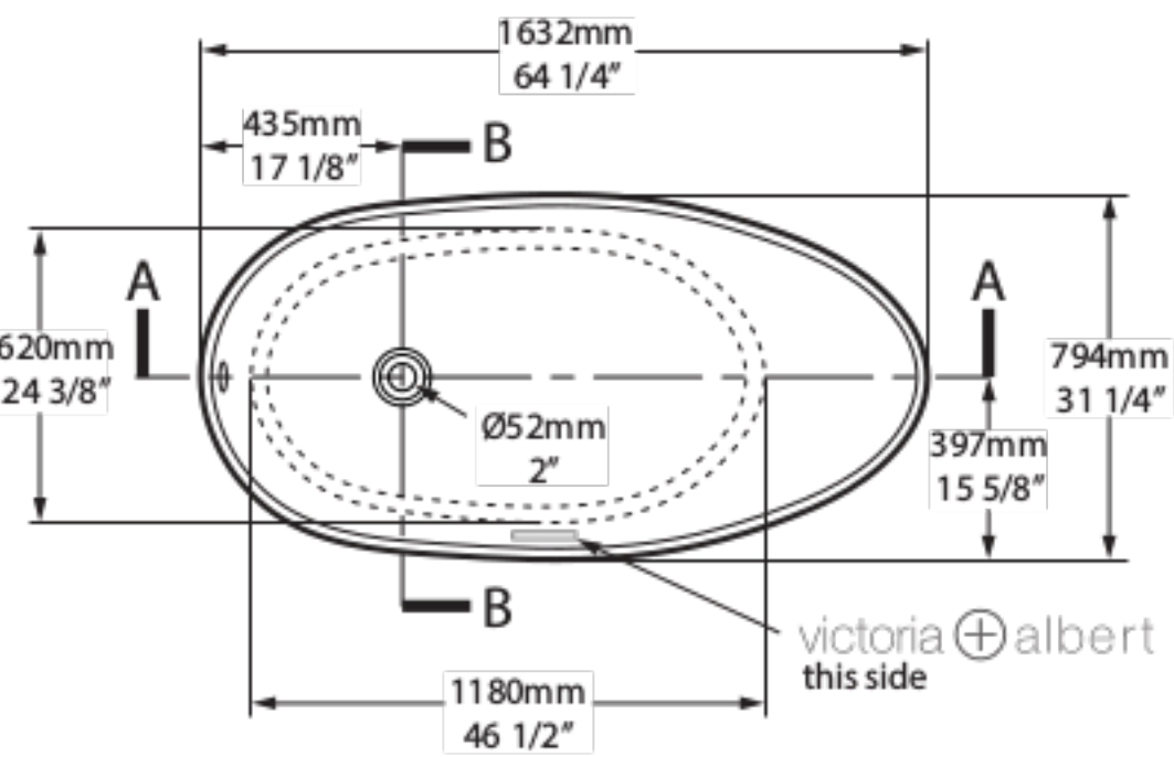
Top View
