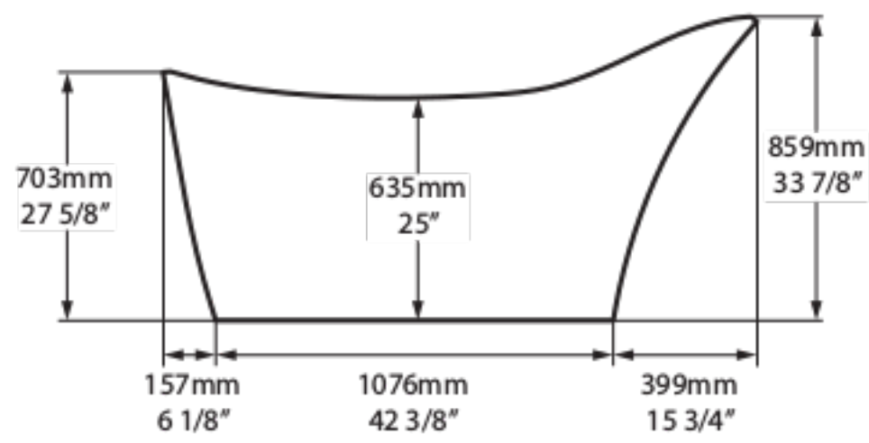
Side View
