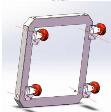
Part10-16pieces
