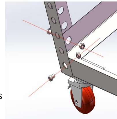
Part5-4pieces
