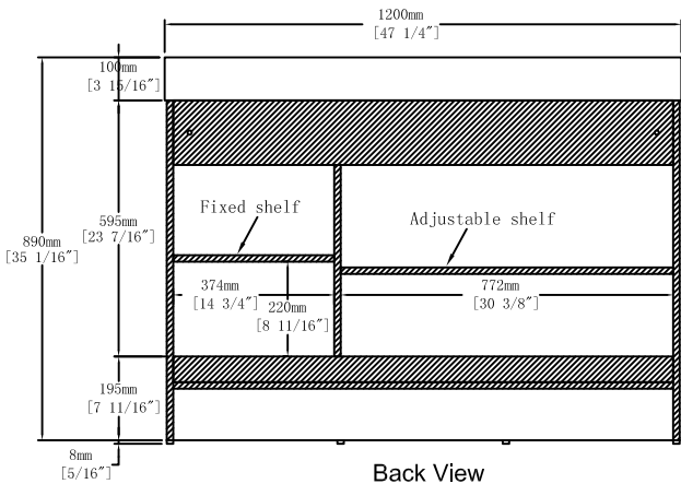
Back View
