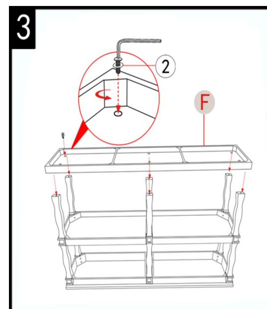
Step 3 Screw the bottom shelf(G) into the legs
