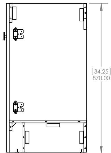
Side View / Vista Lateral
