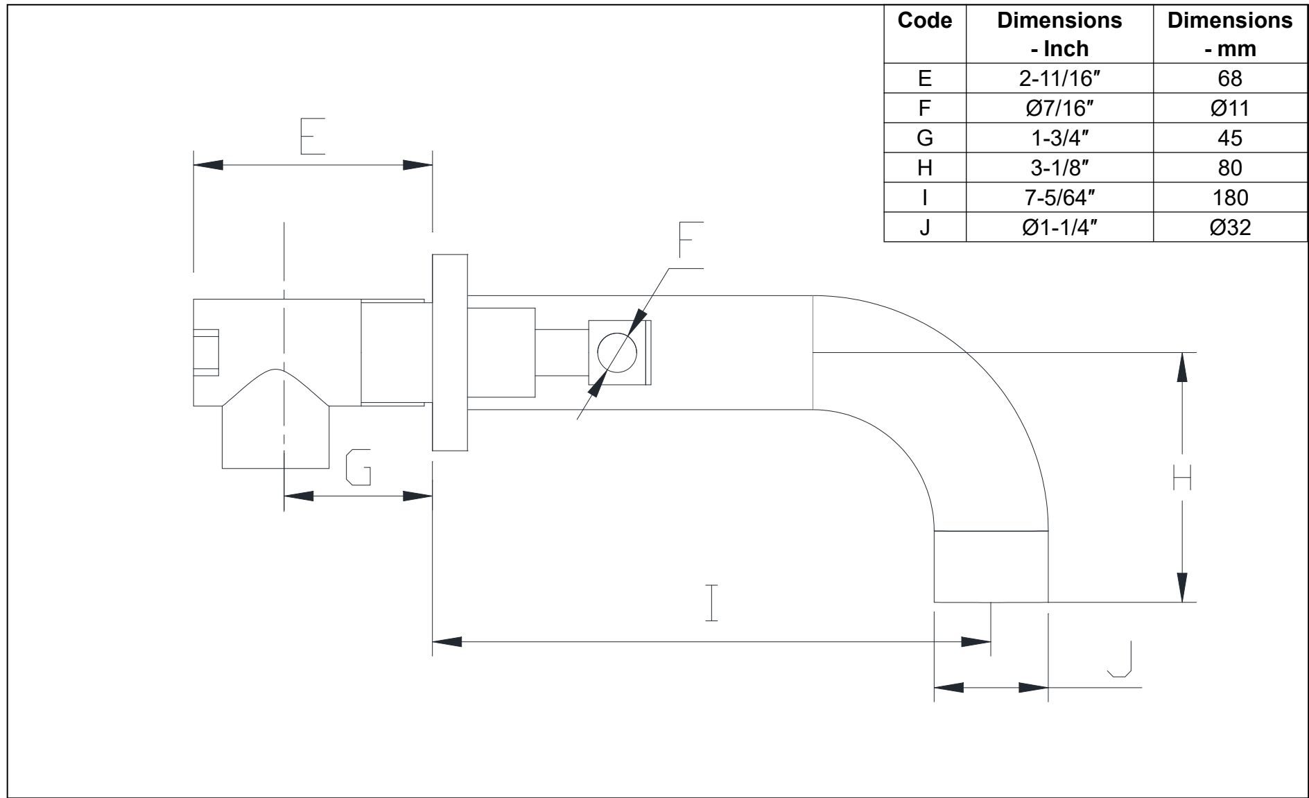
SIDE VIEW
