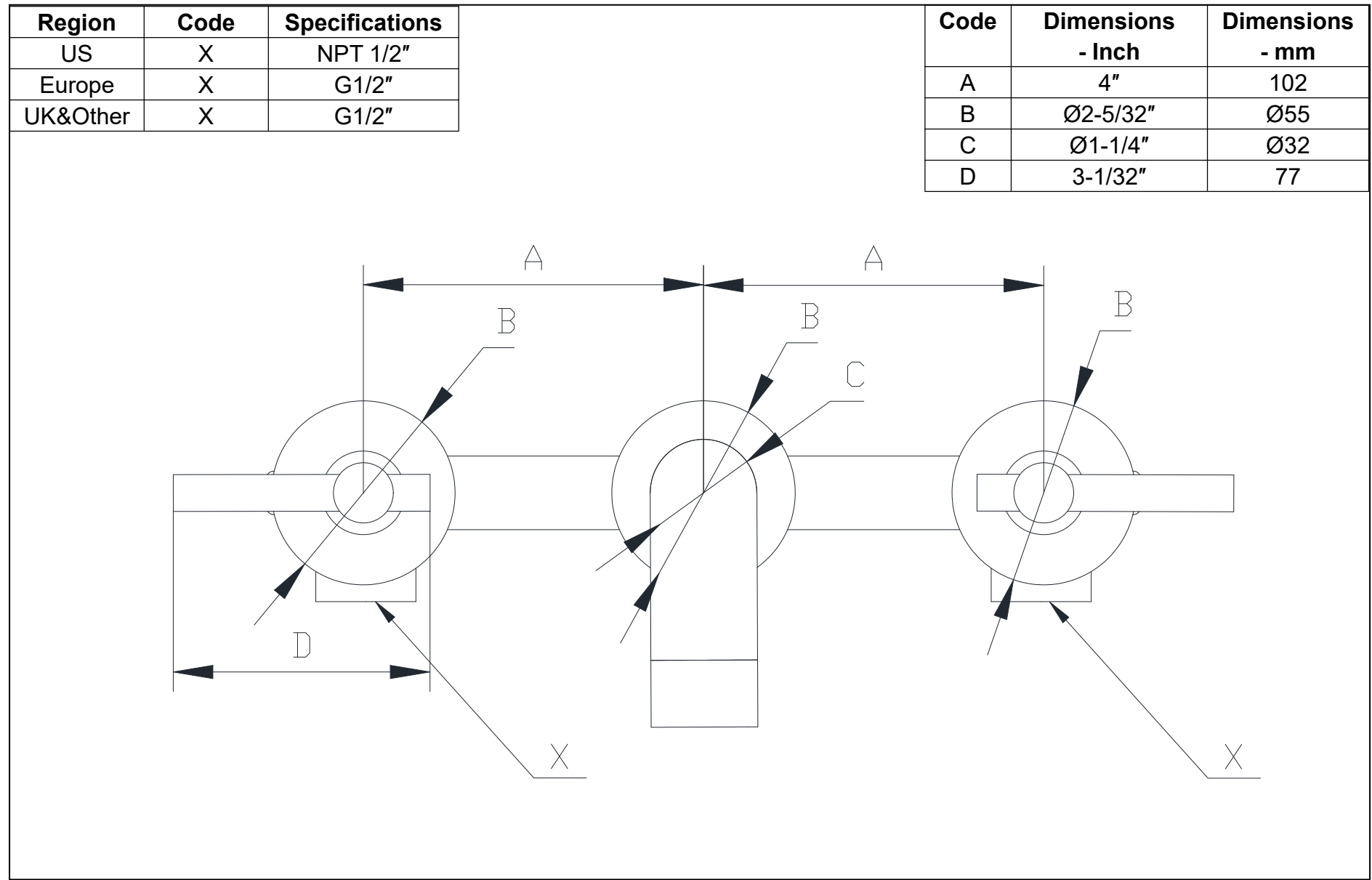
FRONT VIEW
