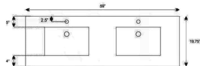
SINK CUT OUT OPENING 15.75"W x 10.75"D
