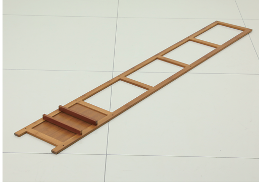
① Position Side Frame (a) and Drawer Slats (n) as picture shown. Secure them with Mid Screws (p).
