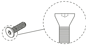
Flat head bolt M6x15mm (8 pcs)
