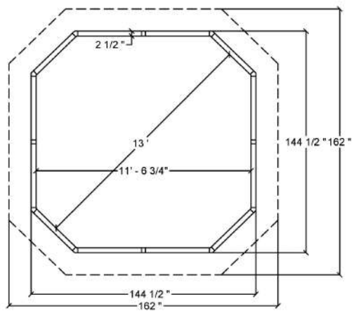
PLAN A LA BASE PLAN AT THE BASE
