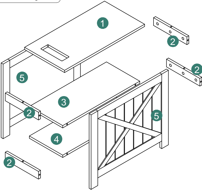
Explosion Diagram
