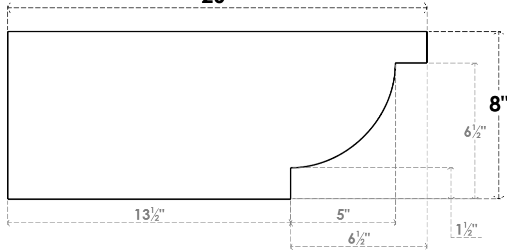
SIDE PROFILE
